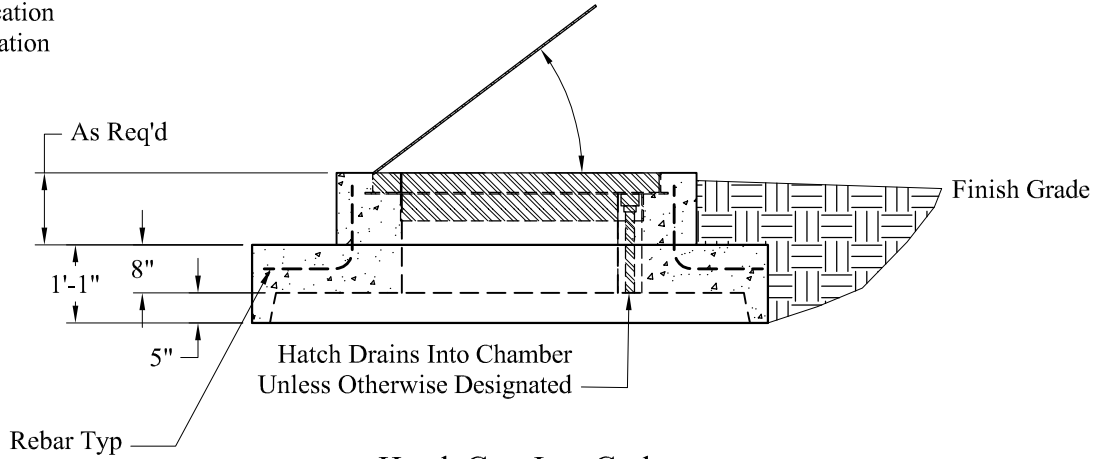
Hatch Cast Into Curb
