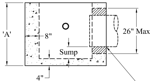
30" Drop Inlet Base
