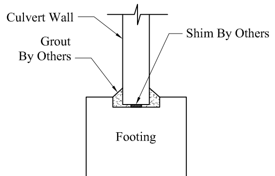
Footing Detail
