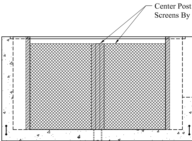
Inlet View
