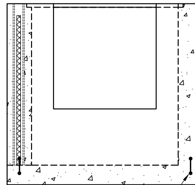
Outlet View
