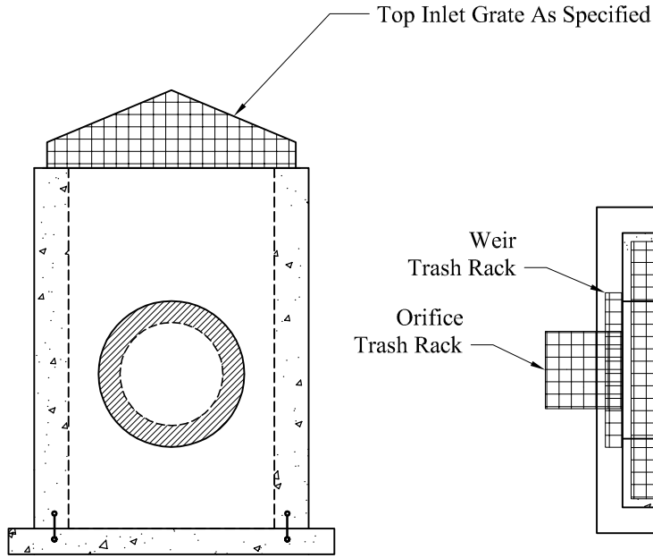
Outlet View
