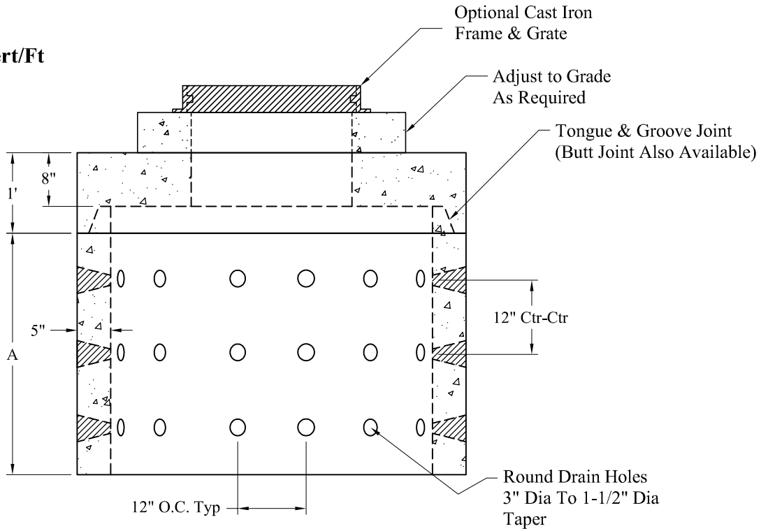
Section View
