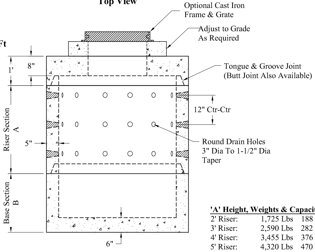
Section View
