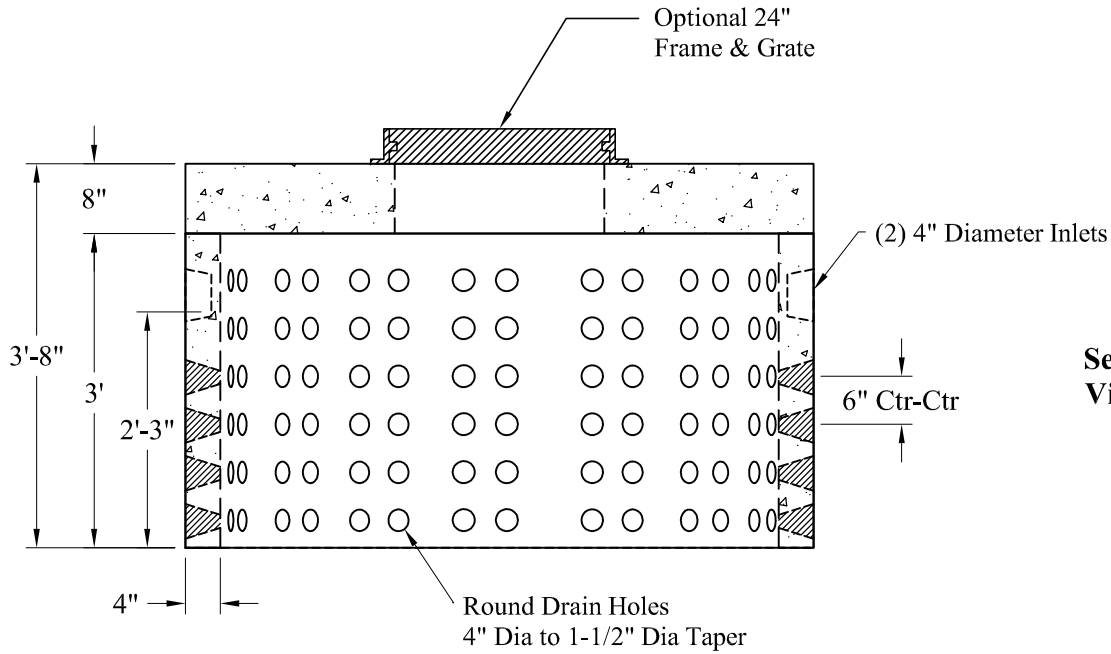
Detail Of Openings (NTS)
