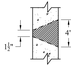
Detail Of Openings (NTS)
