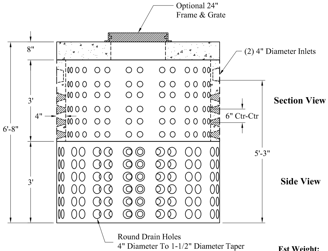
Detail Of Openings (NTS)
