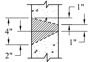
Detail of Openings (NTS)
