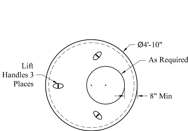
Plan View - Top Slab
