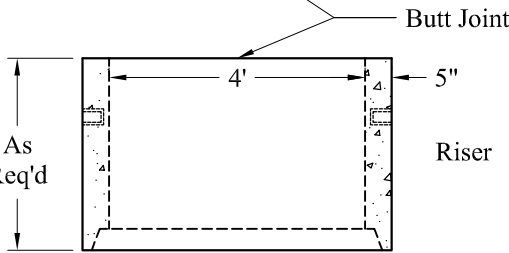
Top Slab
