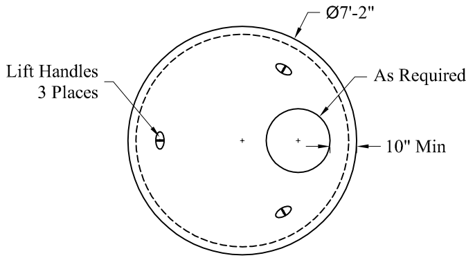
Plan View - Top Slab
