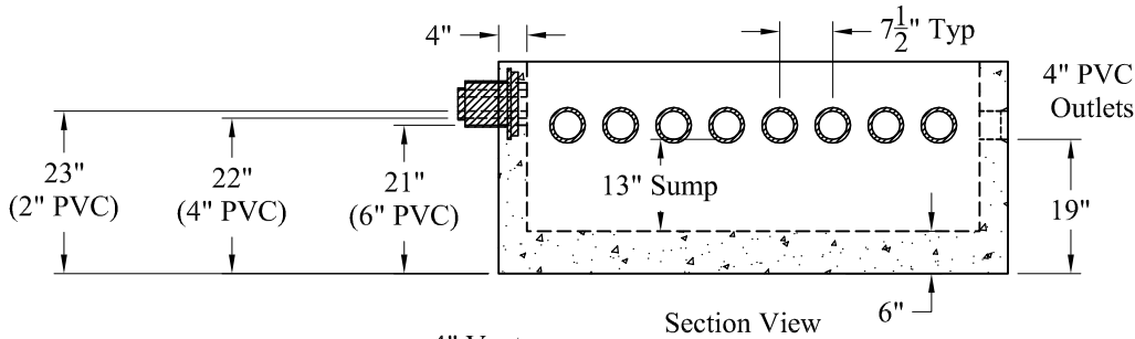
Section View
