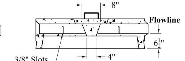
End Section
