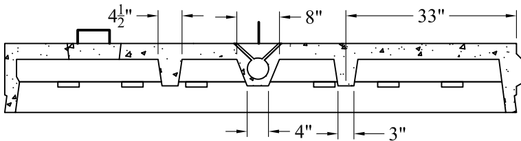
Side Section
