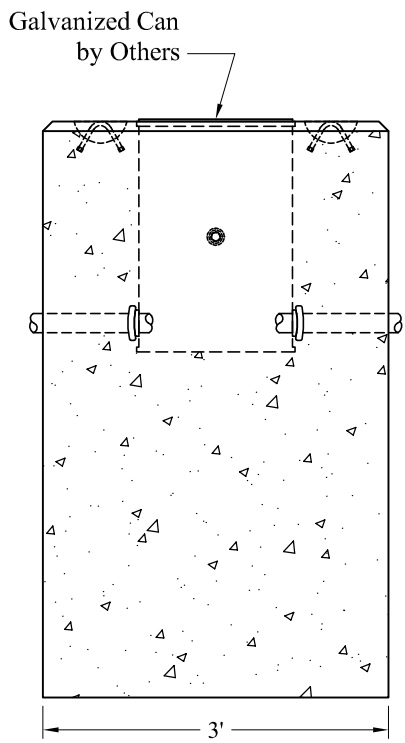
End View
