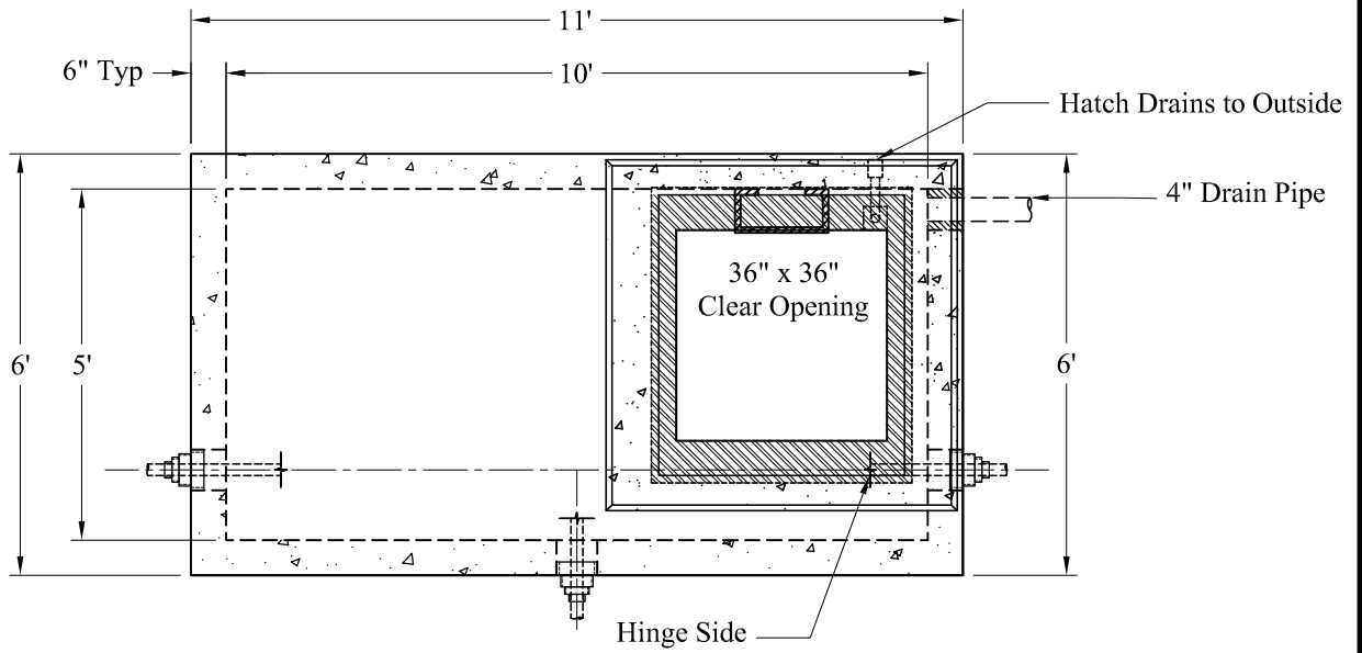
Plan View
