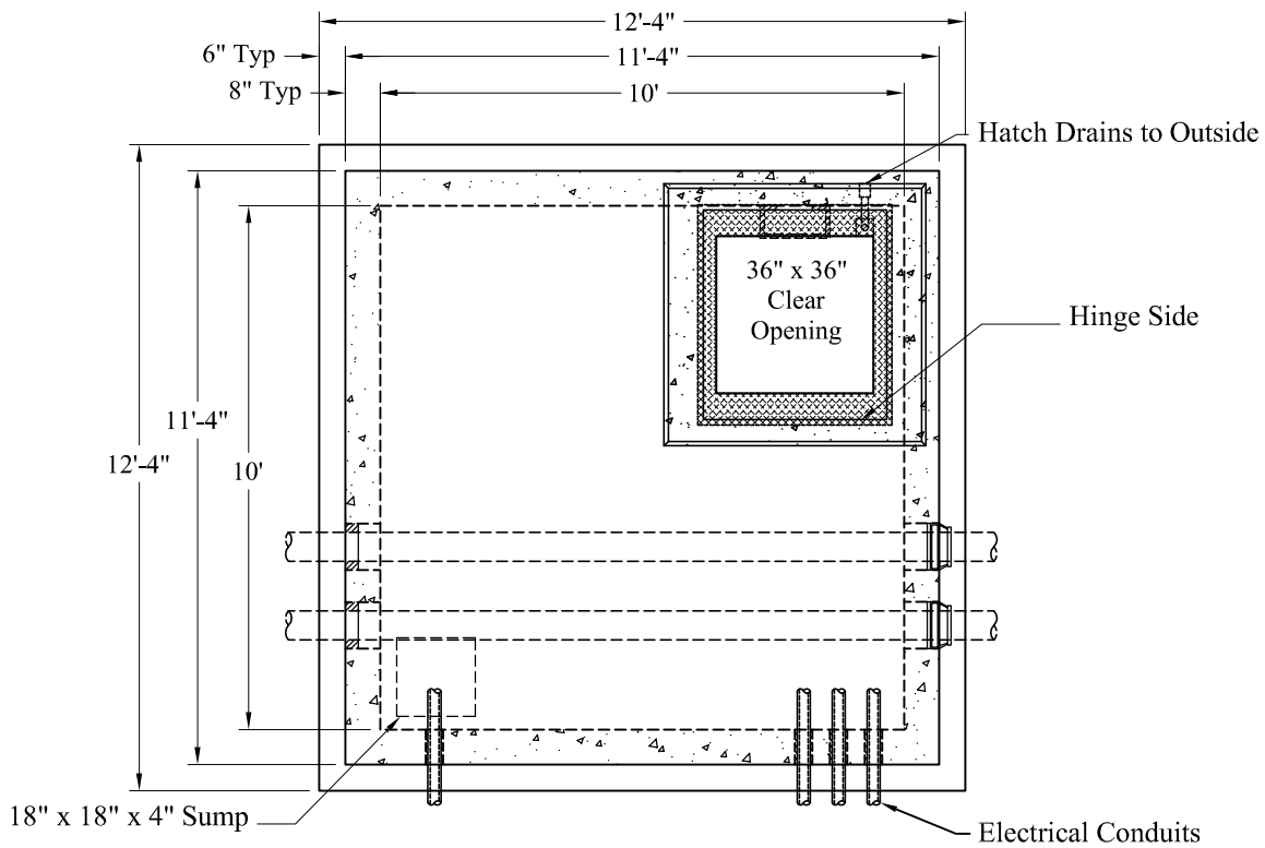
Plan View
