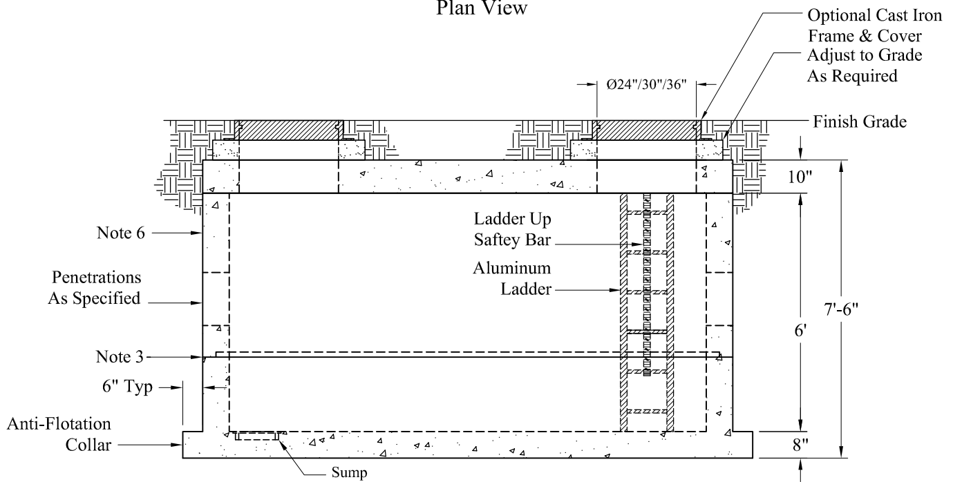
Elevation View
