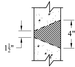
Detail Of Openings (NTS)
