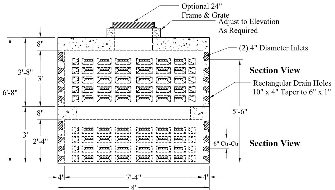
Detail of Openings (NTS)
