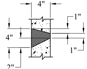
Detail of Openings (NTS)
