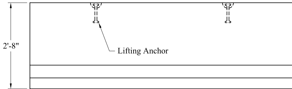
Elevation View
