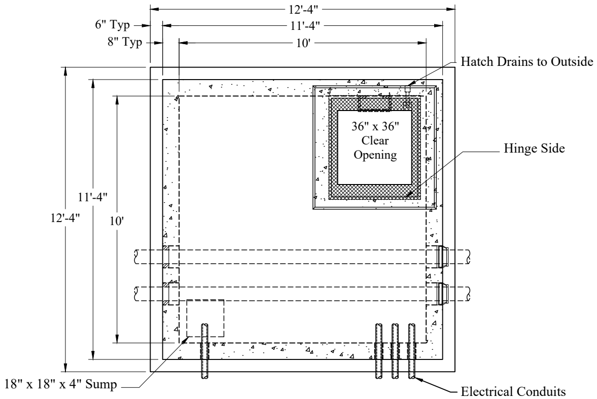
Plan View
