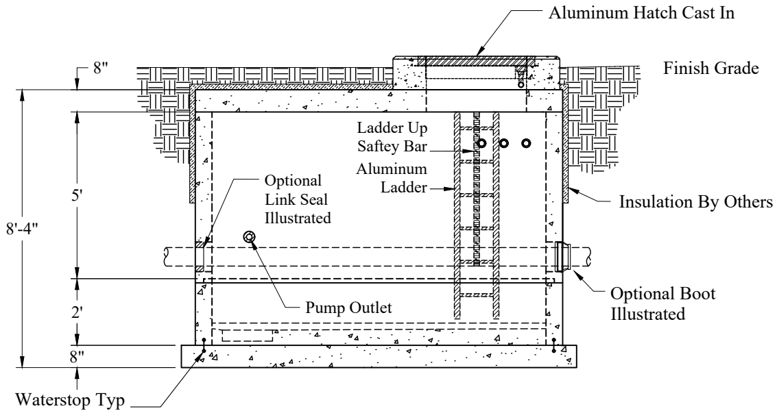
Elevation View
