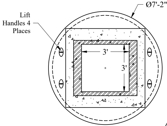
Plan View - Top Slab
