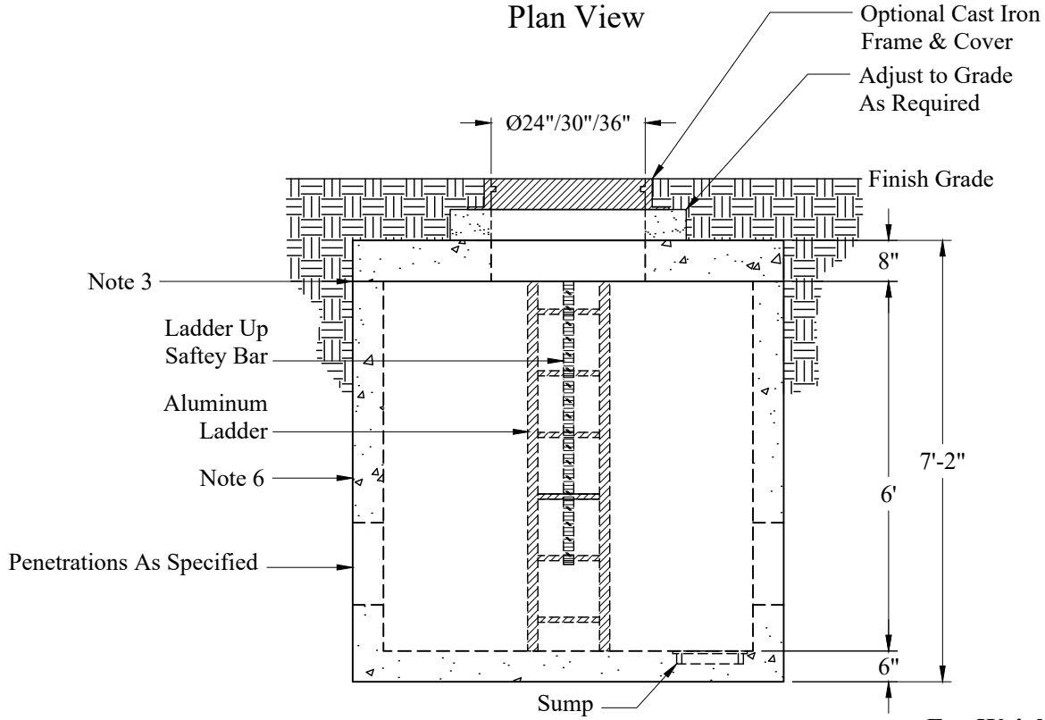
Elevation View
