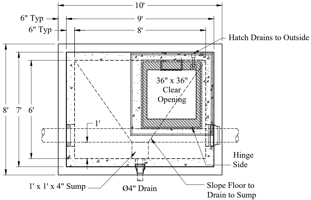
Plan View
