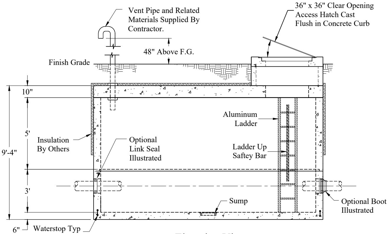
Elevation View
