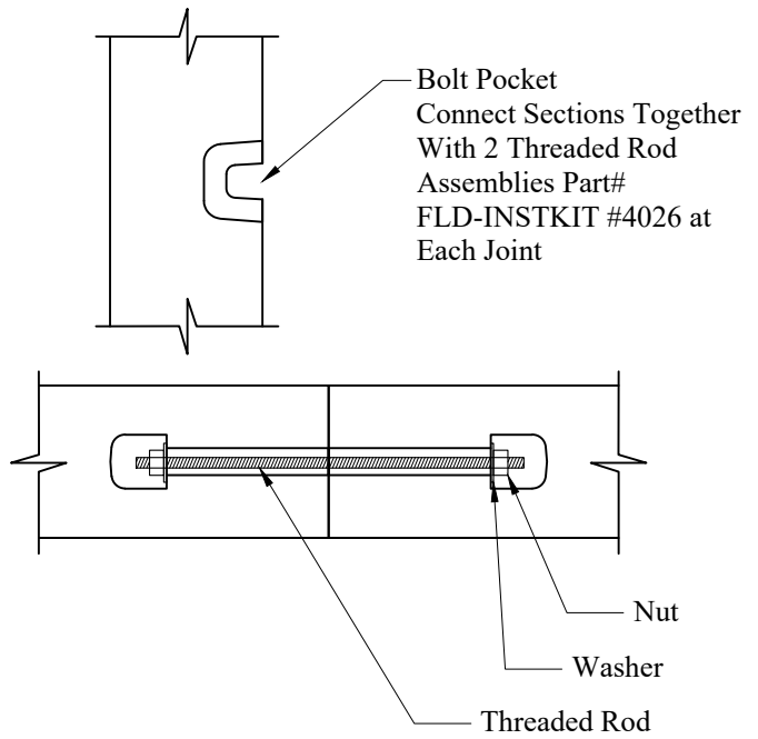
Detail 4 Bolt Pocket Details
