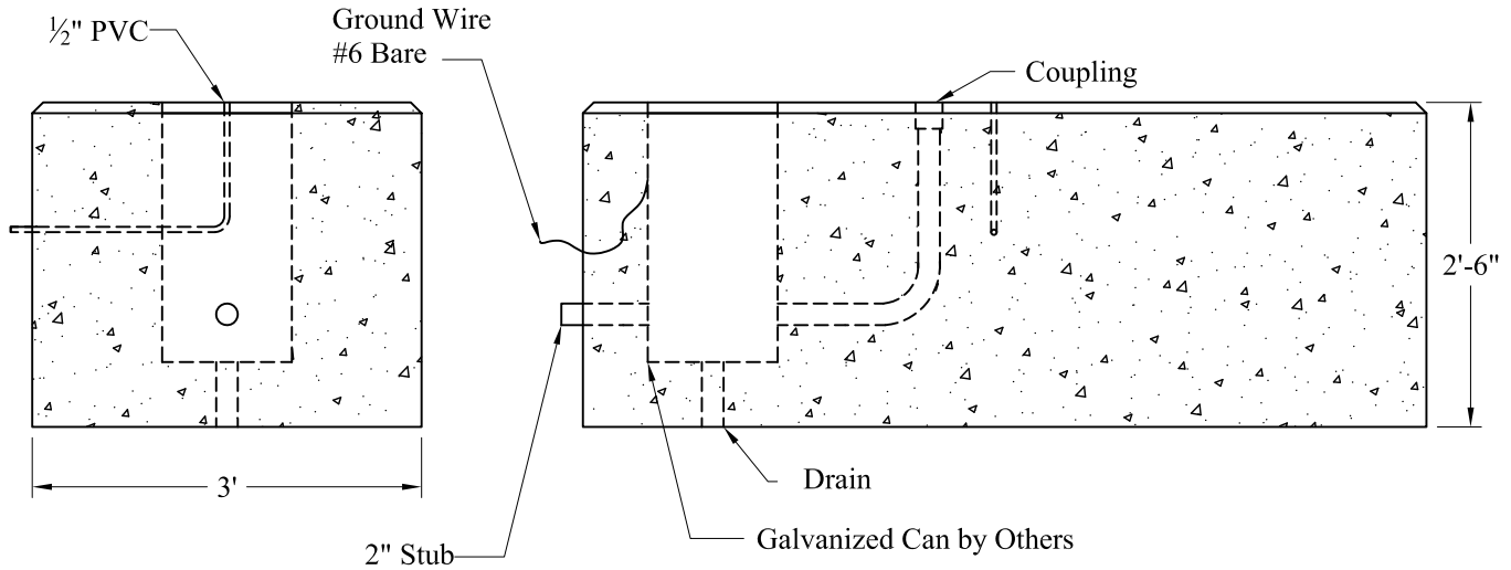
End View
