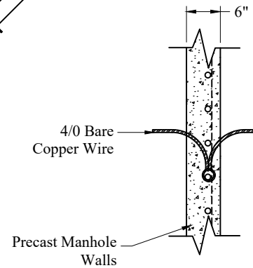
Detail "Y"
