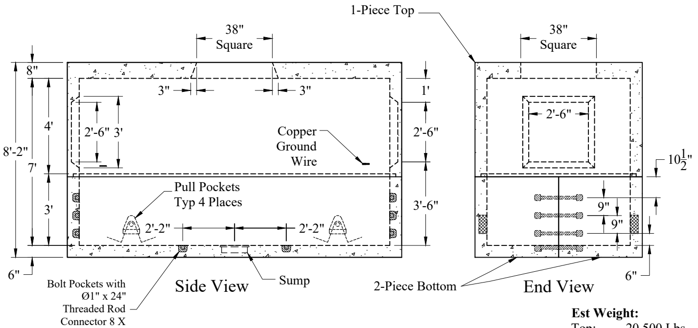
Plan View
