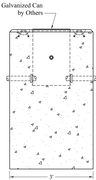
End View
