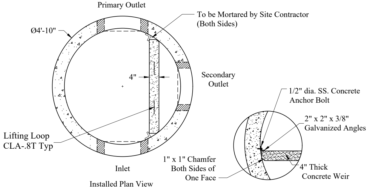
Detail of Mounting Weir to Inner Wall of Structure.
