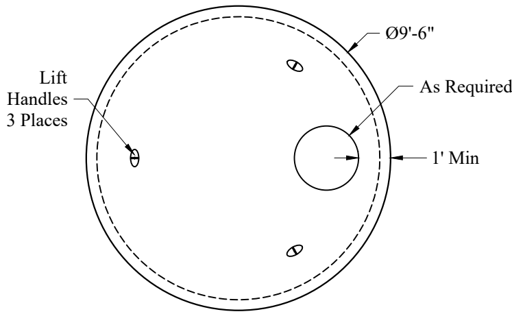
Plan View - Top Slab
