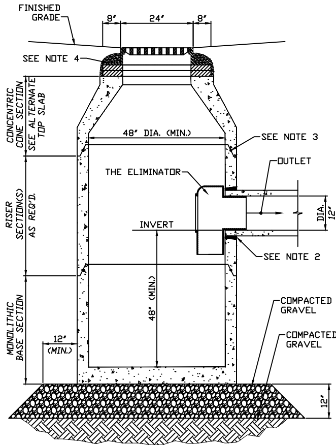
TYPICAL CATCH BASIN (CB) WITH TRAP
