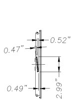
Side View of Cover
