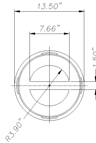
Front View of Cover w/ Integral Handle
