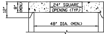
ALTERNATE TOP SLAB
