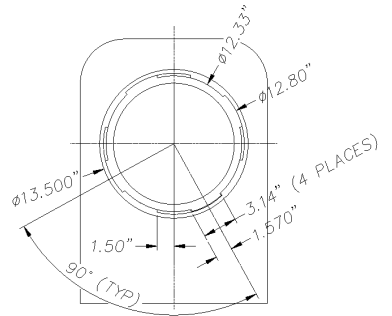
Enlarged Front View
