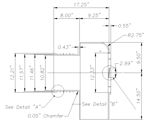
Enlarged Section 1-1
