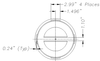
Rear View of Cover w/ Integral Handle
