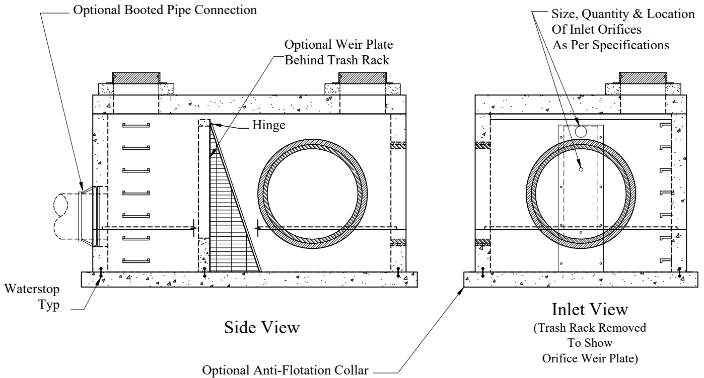
Outlet View
