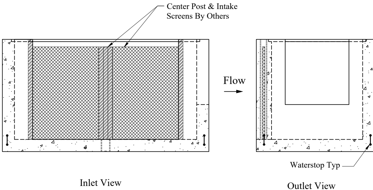
Detail A
