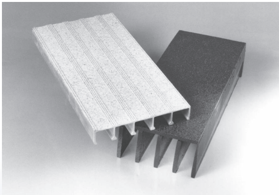
Shown above is a steel grating/solid plate assembly coated with OnGrip® Spray Traction Surface. For applications requiring the light weight or corrosion resistance of an aluminum grating / checkerplate combination, unpunched plank (shown above with OnGrip® Slip Resistant Surface) offers an economical alternative.
