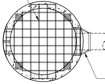
Plan View
