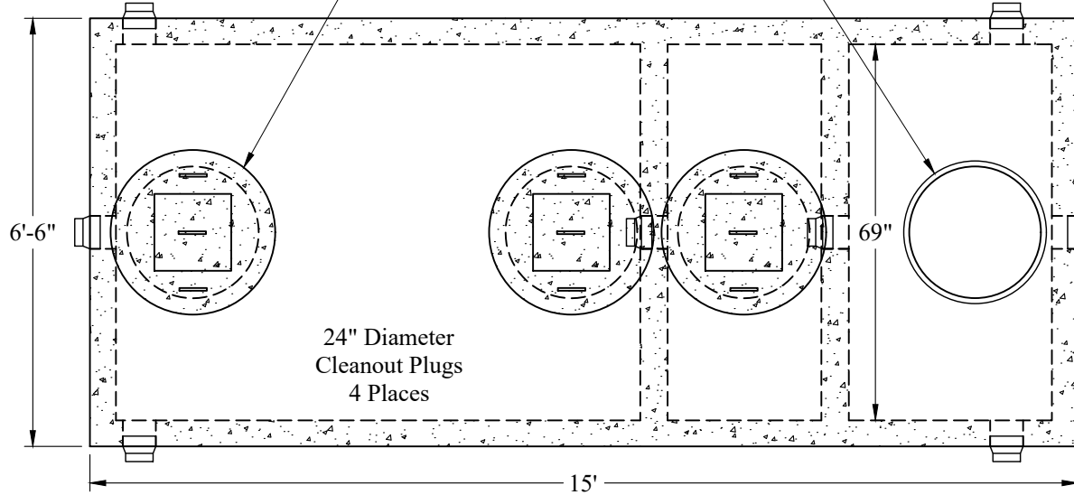
Optional Cover Configuration (4) 24" Dia Plastic Risers Cast In, With Plastic Covers
