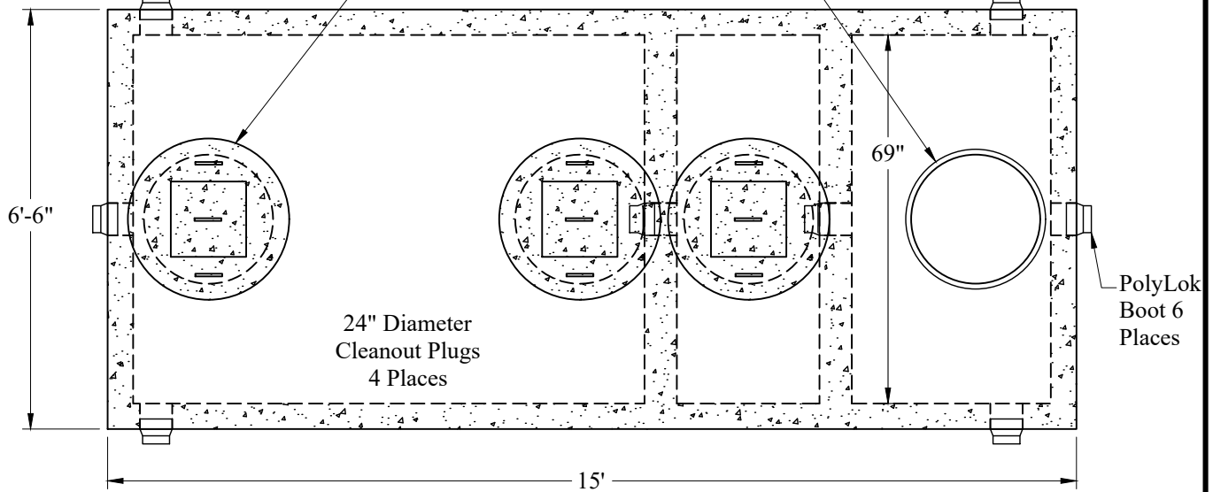
Optional Cover Configuration (4) 24" Dia Plastic Risers Cast In, With Plastic Covers
