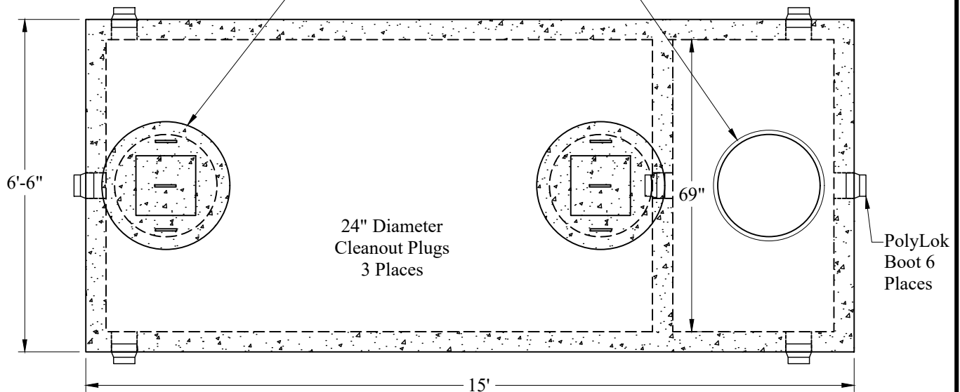
Optional Cover Configuration (3) 24" Dia Plastic Risers Cast In, With Plastic Covers
