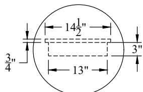
Sump Pan Detail
