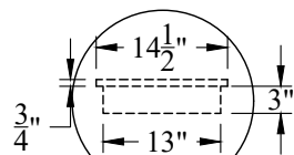
Sump Pan Detail
